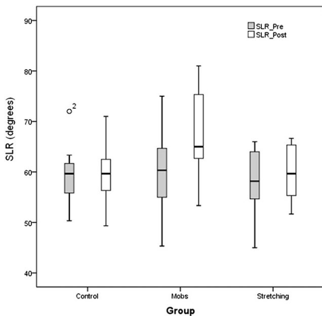
Fig. 2. Clustered boxplot comparing pre-intervention and post-intervention (left and right respectively) SLR measures for each experimental group.
